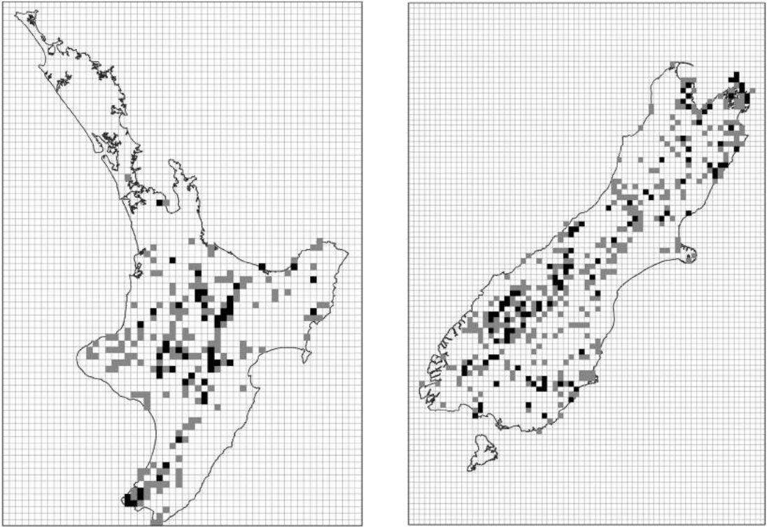
Fig. 2. Breeding distribution of New Zealand falcon on the North Island (left) and South and Stewart islands (right). Lightly shaded squares indicate suspected breeding of falcon; dark shaded squares indicate confirmed breeding of falcon. Each grid squares encloses an area of 10 km x 10 km.
